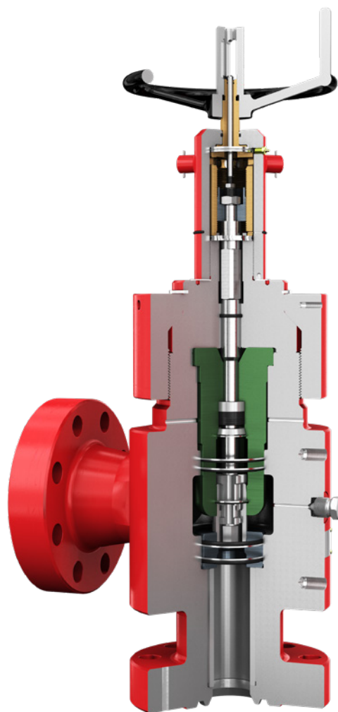
DR20 2-in gate and seat drilling choke.
