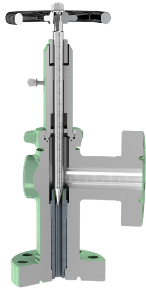
AOP Series BFF* threaded flanged choke.
